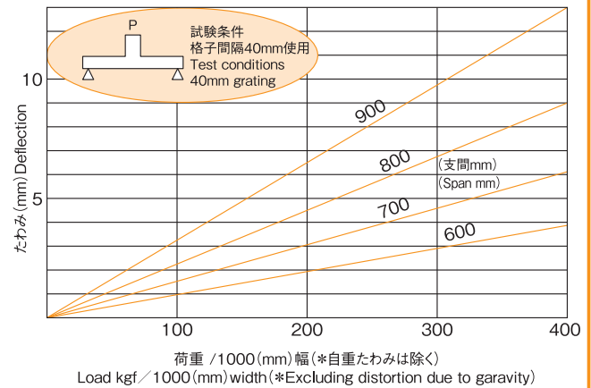
荷重・たわみ線図(中央集中過重) Deflection vs. Load (At center of span)
