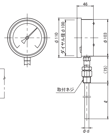
図面 ⑥ LAS-100S
