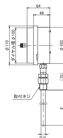
図面 ⑮ LAS-100SE
