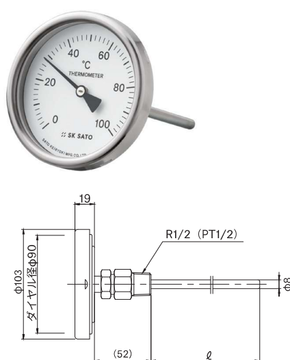
BM-T-90S
