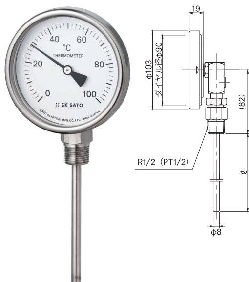
BM-S-90S
