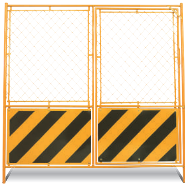
F-18AT (扉) ○ W1800 × H1800mm ○内開き
