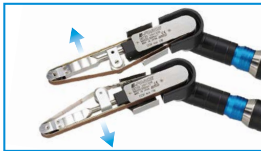
Belt working surface can be reversed 砂带工作面可以颠倒
