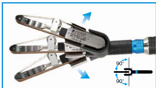
The angle of the belt head can be adjusted 砂带头的角度可以调节
